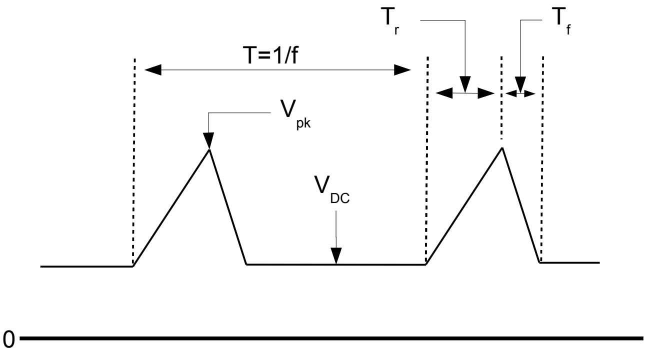
DC-PWM 1/2/3 - Mode 3/4/5
