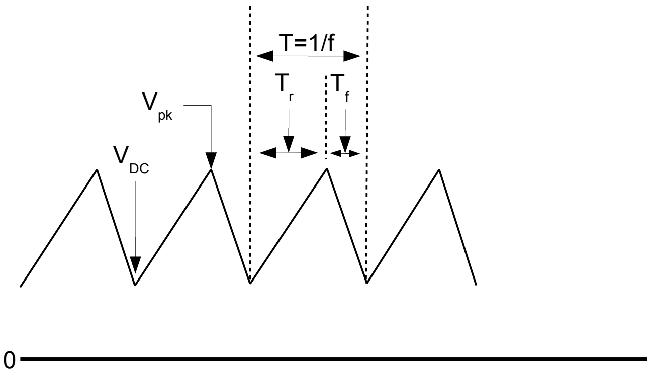
DC-PWM 4 - Mode 6
